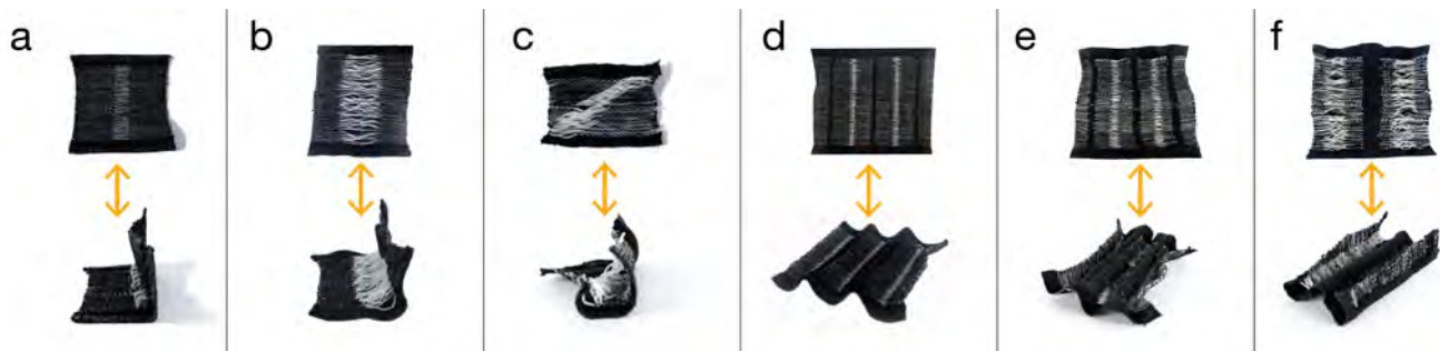
Figure 13: 8cm x 8cm woven samples with FibeRobo; (a) top: a woven piece with nano-plated silver conductive weft threads and a 1.5cm LCE float, bottom: the actuated state; (b) top: a woven sample with a 2.75cm LCE float, bottom: the actuated state; (c) top: a woven sample with a 1.5cm LCE diagonal float, bottom: the actuated state; (d) top: a woven sample with five 0.25 cm floats on alternating sides of the fabric, bottom: the actuated state; (e) top: a woven sample with five 0.5 cm floats on alternating sides of the fabric, bottom: the actuated state; (f) top: a woven sample with five 1 cm floats on alternating side of the fabric, bottom: the actuated state.
