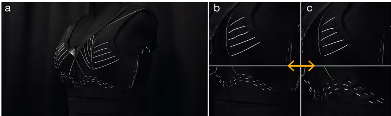
Figure 8: An adaptive support sports bra with hand-sewn continuous FiberoBot patterns. (a) sports bra prototype on a medium-sized mannequin, (b) a close-up image showing the unactuated state, and (c) the actuated state.
