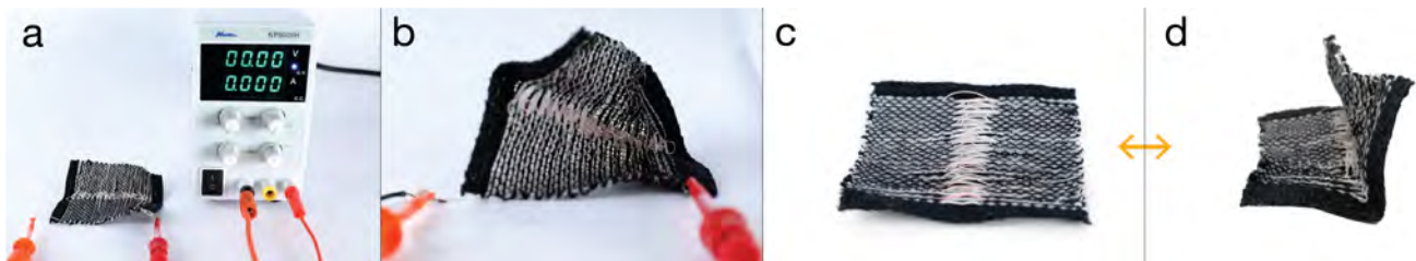
Figure 14: Demonstration of how heat actuation influences the form characterization of woven fabric samples using LCE fibers with float lengths of 1.5cm. (a) demonstration of heating set up; (b) fabric form response to 2.5 amps and 4 V; (c) closeup of the unactuated state; (d) closeup of the actuated state
