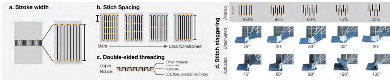
Figure 10: (a) Stroke width, (b) Stitch spacing, (c) Double-sided threading, and (d) Staggered stitches lead to different folding angles.
